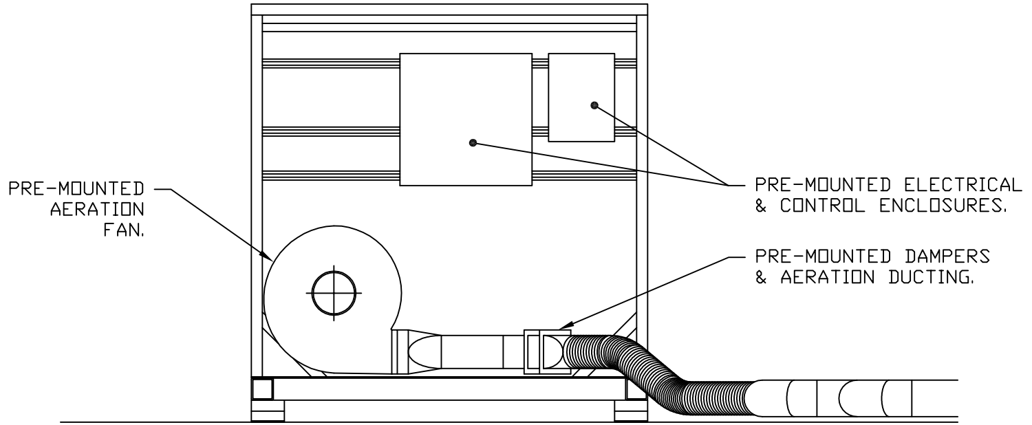
AERATION SKID ELEVATION SCALE: 1/2"=1'
