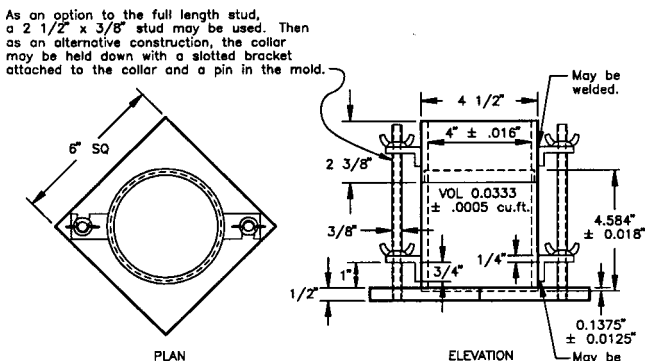
FIG. 1 4.0-in. Cylindrical Mold
