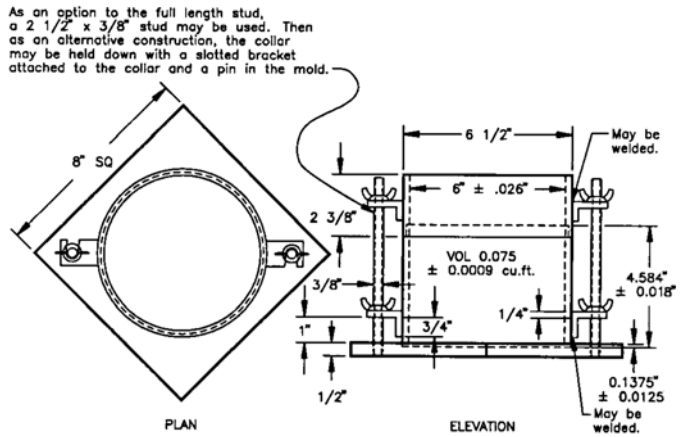
FIG. 2 6.0-in. Cylindrical Mold
