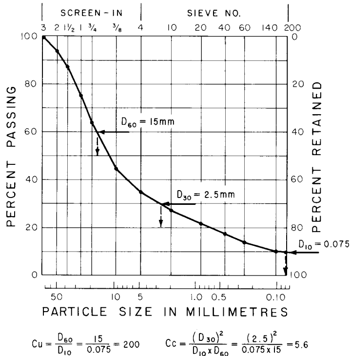
FIG. 5 Cumulative Particle-Size Plot
